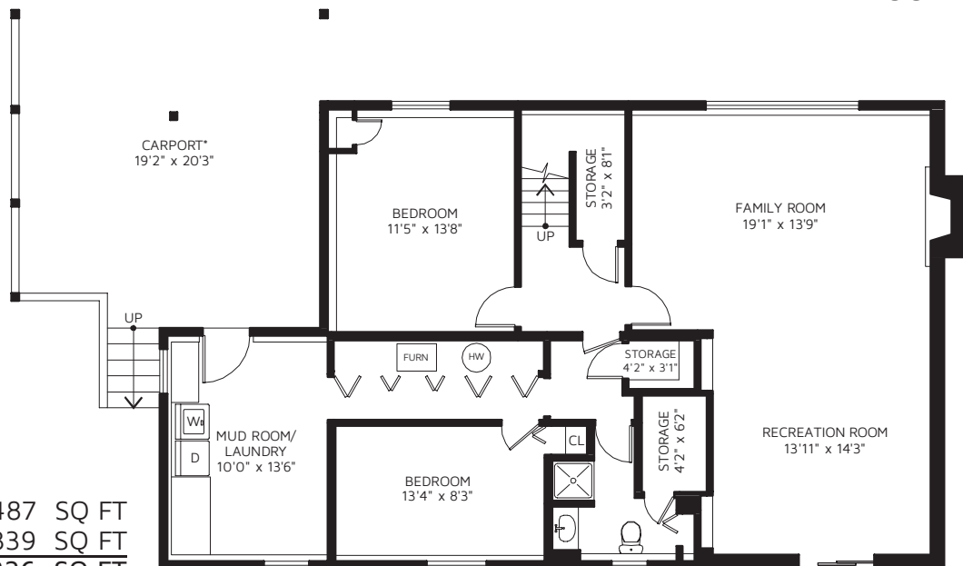
BASEMENT
