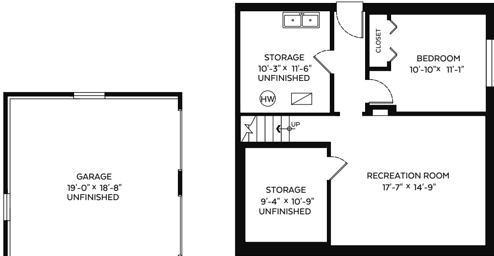
Lower Floor Plan Floor Area: 845 sq.ft.
