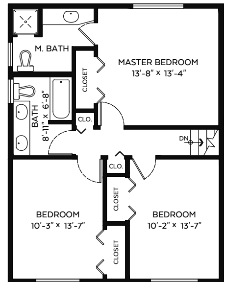
Upper Floor Plan Floor Area: 772 sq.ft.
